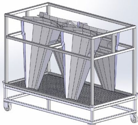
Outlet chutes in the cleaning trolley
