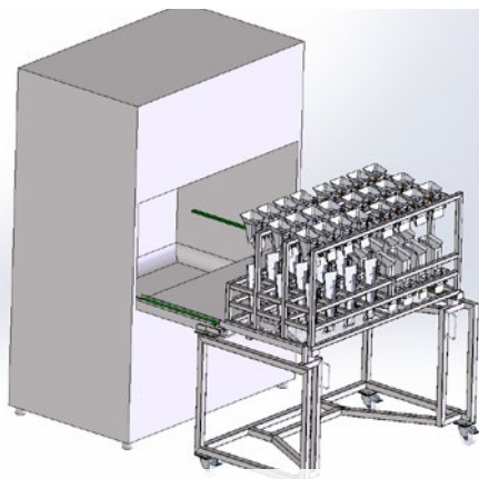
Cleaning trolley and washing machine
