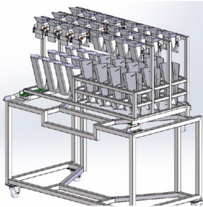
Pool- and weighhoppers in the cleaning trolley
